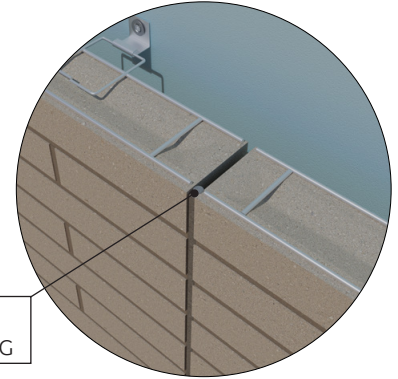
CONTROL JOINT DETAIL
