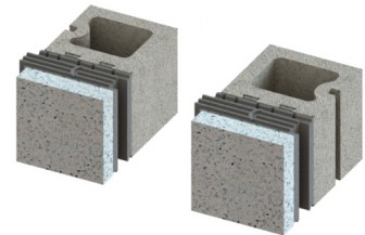
Half Sash Unit - Left/Right
