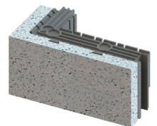
Left Hand L-Corner Unit Face With Profiled Insert For First Row
