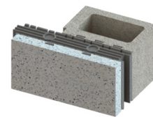
Right Hand Corner Continuation Unit
