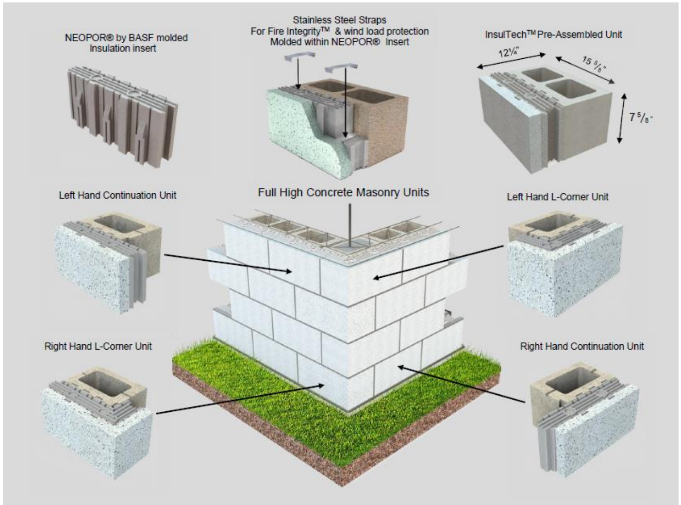
Figure 1. Full Height Typical Details
