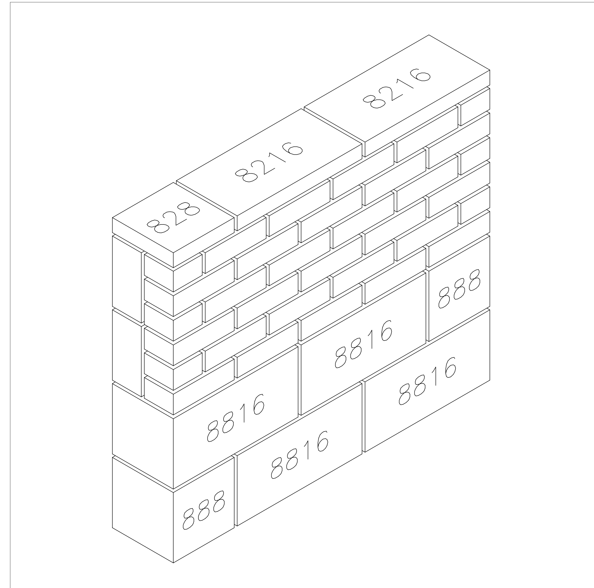
1 ISOMETRIC VIEW SCALE: NONE REF:
