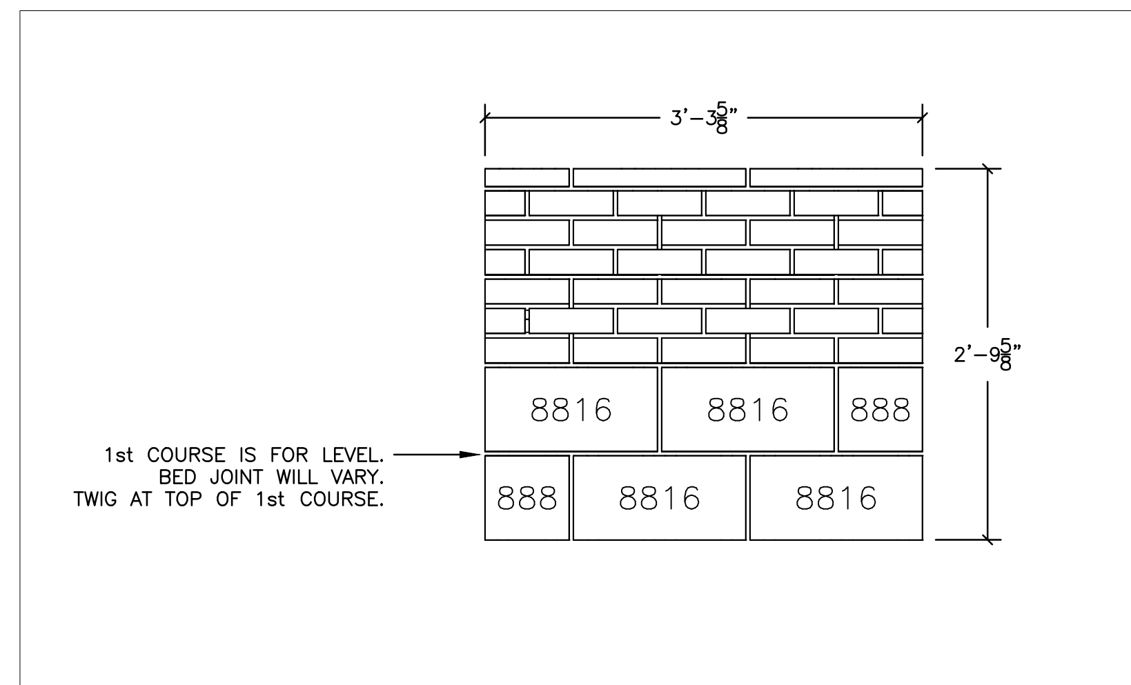
3 FRONT ELEVATION SCALE: 1" = 1" REF:
